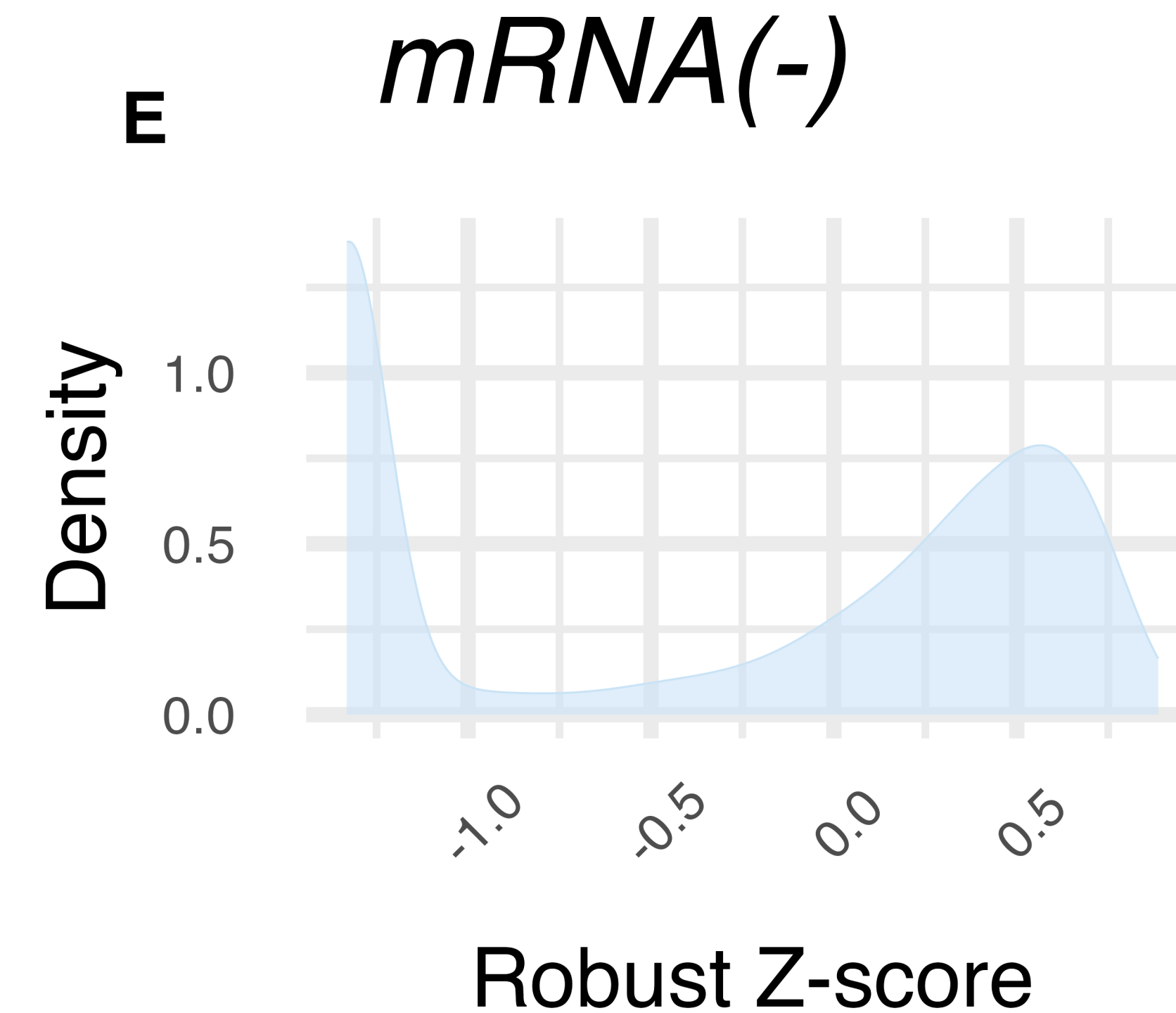
Supplementary Figure S7. mRNA methylome robust z-scores distributions in log scale. A-C) Histogram, Density and Boxplot for mRNA(+), D-F) Histogram, Density and Boxplot for mRNA(-). The positive dataset shows robust z-scores centered around 0.5 and the robust z-scores for the negative set are centered around 0, this indicates that the two datasets come from different distributions. *Note: These distributions highlight the presence of two z-score peaks, which are also distinguished in the main paper figure (Fig 4).
